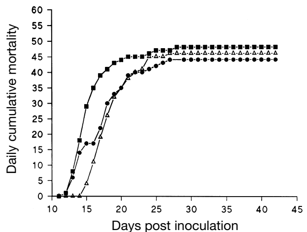
Fig. 2. Percent cumulative mortality of Atlantic salmon in freshwater after intraperitoneal and oral inoculation (total dose 10^{3.5} TCID 50 ) with different ISAV isolates. (■) HKS-36 virus grown in SHK-1 cells; (▲) HKS-36 virus grown in CHSE-214 cells; (●) 'Site A 98' virus grown in CHSE-214 cells
